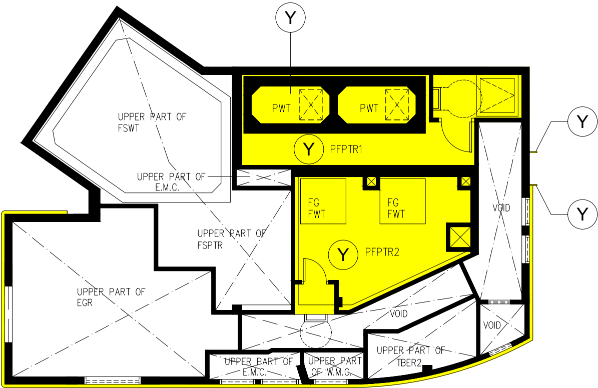
UPPER ROOF PLAN
