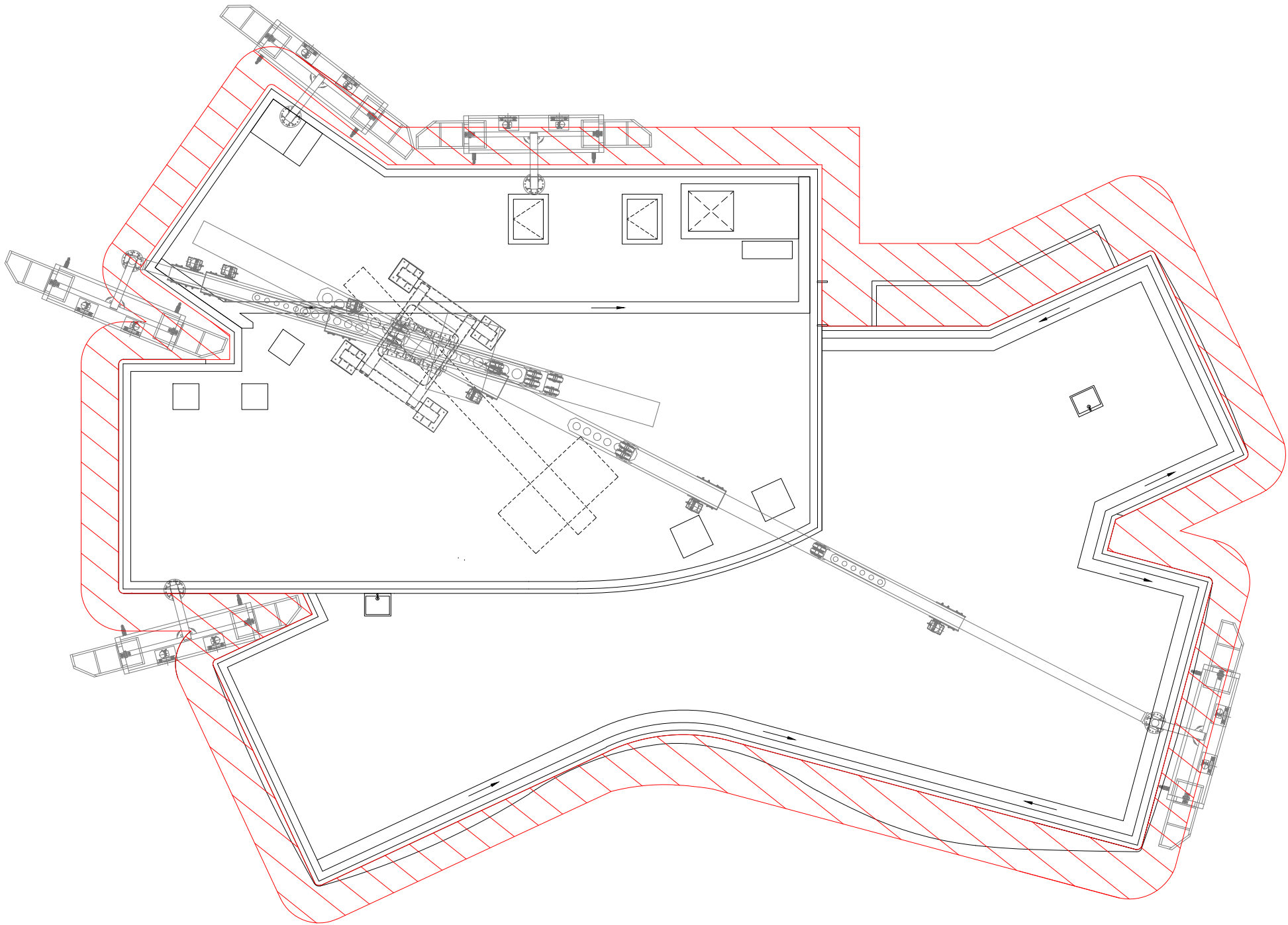
M&R PLAN – ROOF LAYOUT PLAN (CRADLE WORKING)
